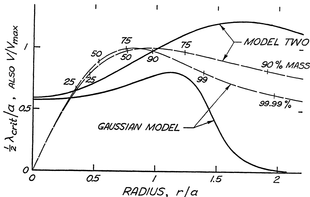
FIG. 1.—Locally estimated critical wavelengths, \lambda_{crit} , for two galaxy models, as functions of the radius (and divided by 2 for plotting purposes). The broken curves describe the rotation laws for these models, and the vertical marks identify the radii which contain the indicated percentages of their respective total masses.
