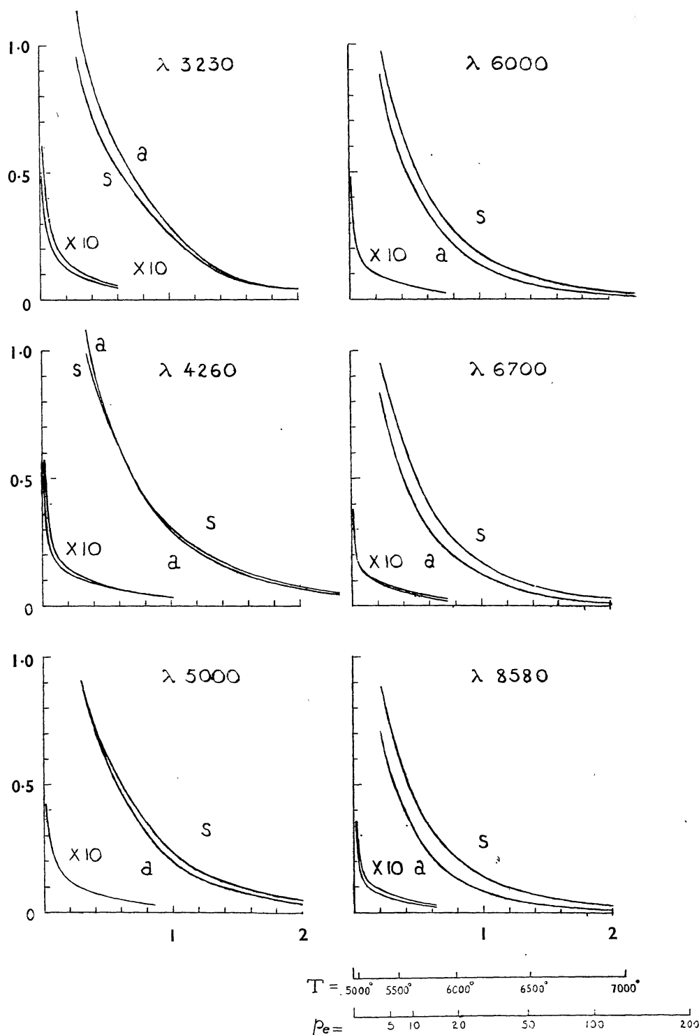
FIG. 4.—Weighting functions h_1(\tau) , h(\tau) .
