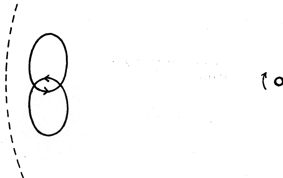
FIG. 4.—Relative Orbits in the Galactic Plane.
