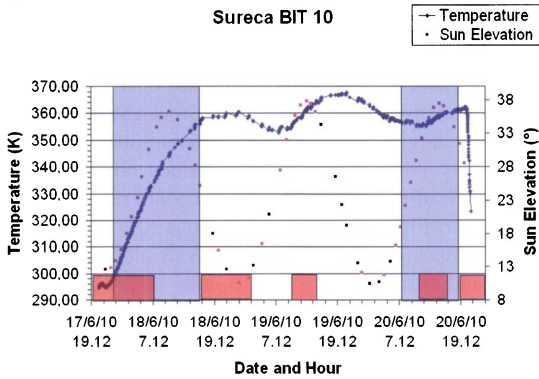
Figure 5. BIT motherboard temperature during the flight in relation with the Sun elevation, the scientific instrumentation ON periods (red boxes) and navigation
