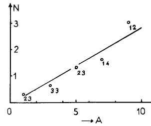
Figure 18: Plot of the average number of bursts observed per day ( N ) versus the average amplitude of fringes ( A ) near local noon, expressed as a percentage of total solar radiation. The number of days used in calculating the various points are listed beside the points (after Kundu, 1959a: 225).
