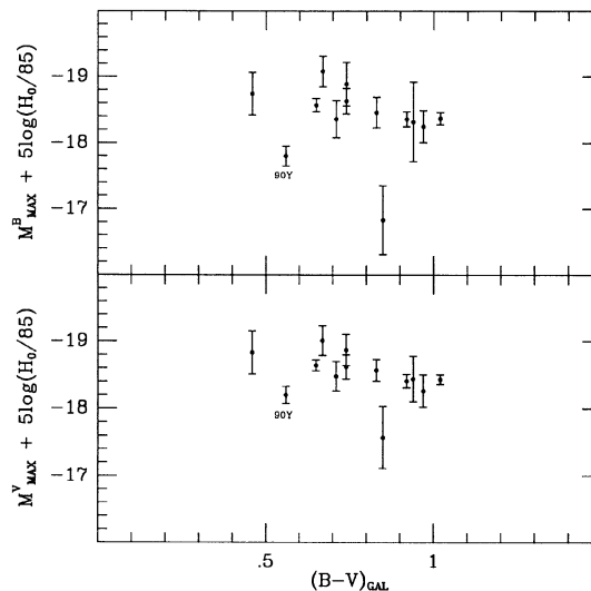
FIG. 8. The absolute B and V magnitudes of the Calán/Tololo SNe Ia plotted as a function of the integrated B-V colors of their host galaxies.
