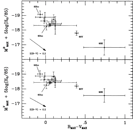
FIG. 3. The absolute B and V magnitudes of the Calán/Tololo sample of 13 SNe Ia, plotted as a function of their B_{\text{MAX}} - V_{\text{MAX}} colors. The galactic reddening vectors (with slopes of 4 in B , and 3 in V ) corresponding to E(B - V) = 0.2 are indicated.
