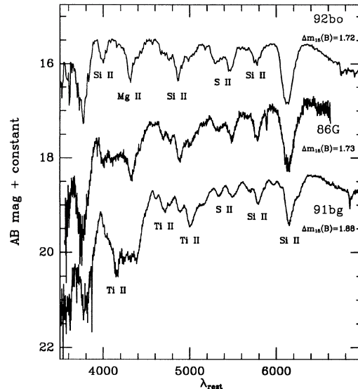
FIG. 6. Comparison of the maximum light spectra of the fast-declining SNe 1992bo, 1986G, and 1991bg. Note the subtle spectroscopic differences in the region of the Ti II absorption between SNe 1992bo and 1986G in spite of the identical initial decline rates of the B light curves.
