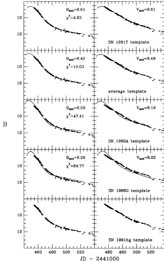
FIG. 13. Fits of the B and V photometry of SN 1972E to five template light curves selected to represent the full range of post-maximum decline rates observed for SNe Ia. Note that fits to the SN 1991bg template are not shown since the \chi^2 minimizing procedure did not converge to a reasonable initial solution.
