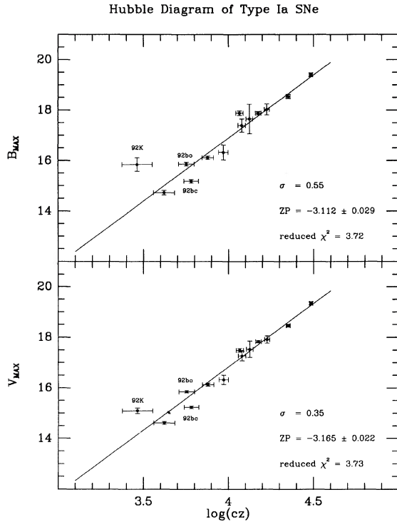
FIG. 2. The Hubble diagrams in B and V for the 13 Calán/Tololo SNe Ia reduced to date.
