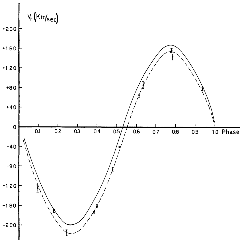
Fig. 1. Radial velocity curve derived by the SiIII lines. The full line represents the observations by SAHADE et al.
