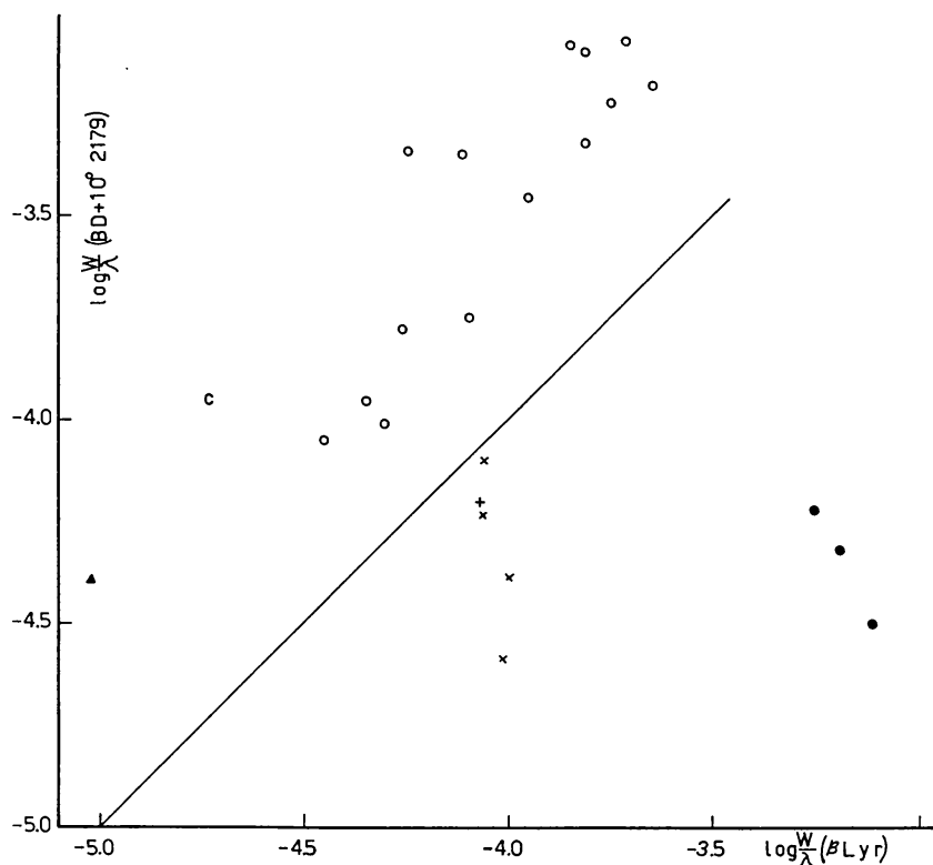
Fig. 6. Comparison of the equivalent widths for BD + 10° 2179 and \beta Lyr. \bullet H I; \circ He I; \odot C II; + Mg II; \times Si II; \blacktriangle Si III
