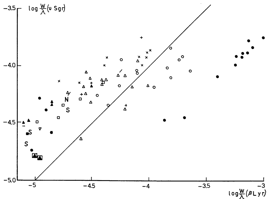
Fig. 5. Comparison of the equivalent widths for \nu Sgr and \beta Lyr. \bullet H I; \circ He I; \ast S II; + N II; + Mg II; \times Si II; \otimes Si III; \nabla Sc II; \square Ti II; \blacksquare V II; \blacktriangle Cr II; \blacktriangle (im Quadrat) Fe I; \triangle Fe II; \triangle (im Kreis) Fe III; / Ni II; - Sr II
