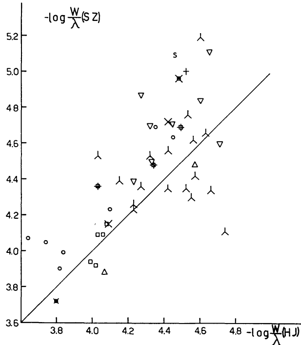
Fig. 2. Comparison of the equivalent widths measured by us and by STRUVE and ZEBERGS. \circ He I; \times N II; \triangle Mg II; \square Si II; \star Ca II; \boxtimes Sc II; \nabla Ti II; \blacktriangledown Cr II; + Fe I; \lambda Fe II; \oplus Ni II; S Sr II.
