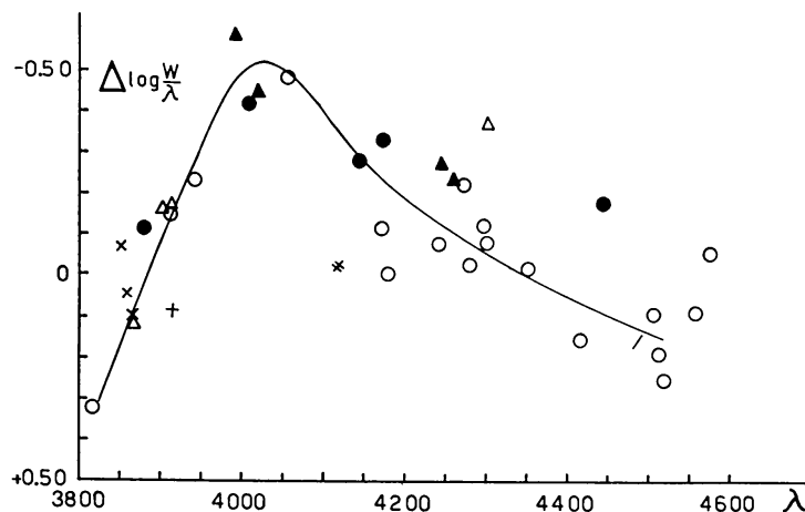
Fig. 3. \log \frac{W}{\lambda} (SZ) — \log \frac{W}{\lambda} (HJ) (indicated with \Delta \log \frac{W}{\lambda} ) versus \lambda . ● HeI: / MgII; × SiIII; + CaII, △ TiII; ▲ CrII; ○ FeII
