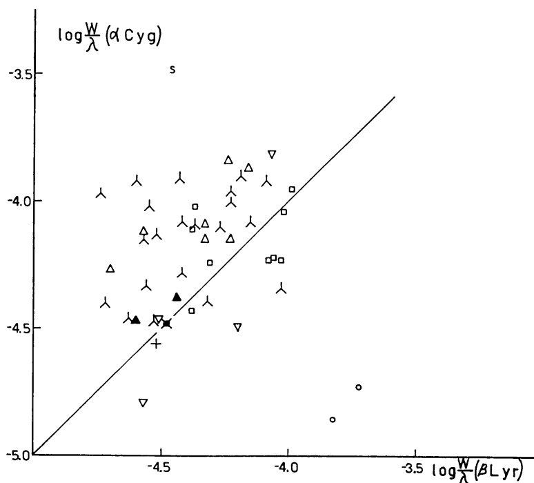
Fig. 4. Comparison of the equivalent widths for \alpha Cyg and \beta Lyr. ○ HeI; ▽ MgII; □ SiIII; × ScII; △ TiII; ▲ CrII; + FeI; λ FeII; S SrII
